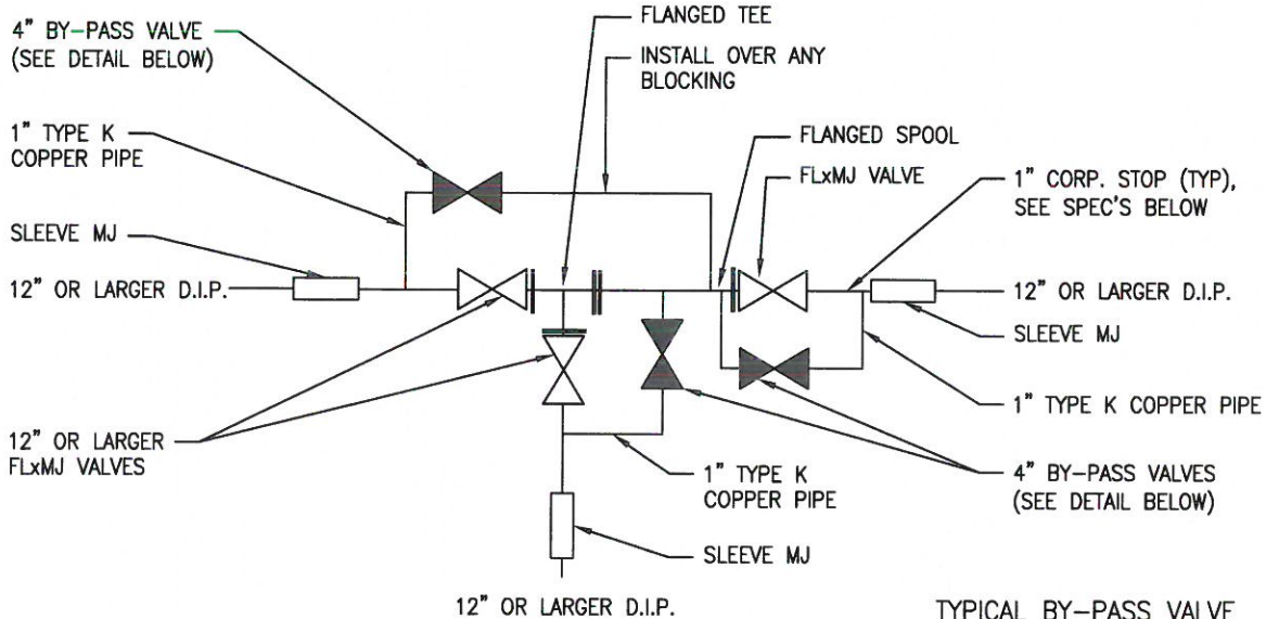
TYPICAL BY-PASS VALVE PLACEMENT
