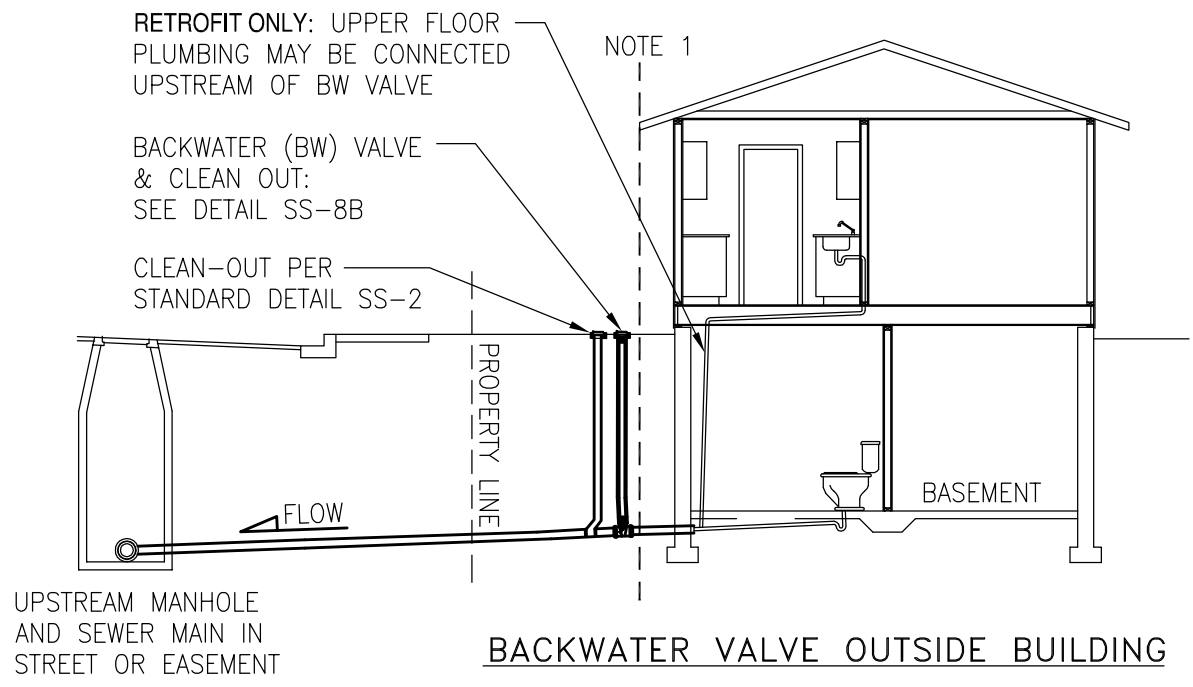
BACKWATER VALVE INSIDE BLDG/BASEMENT
